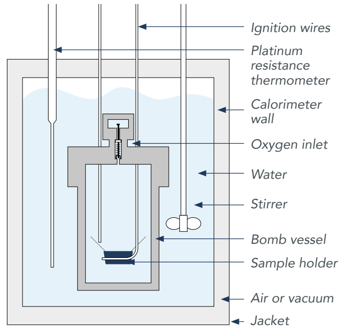
Oxygen Bomb Calorimeter
