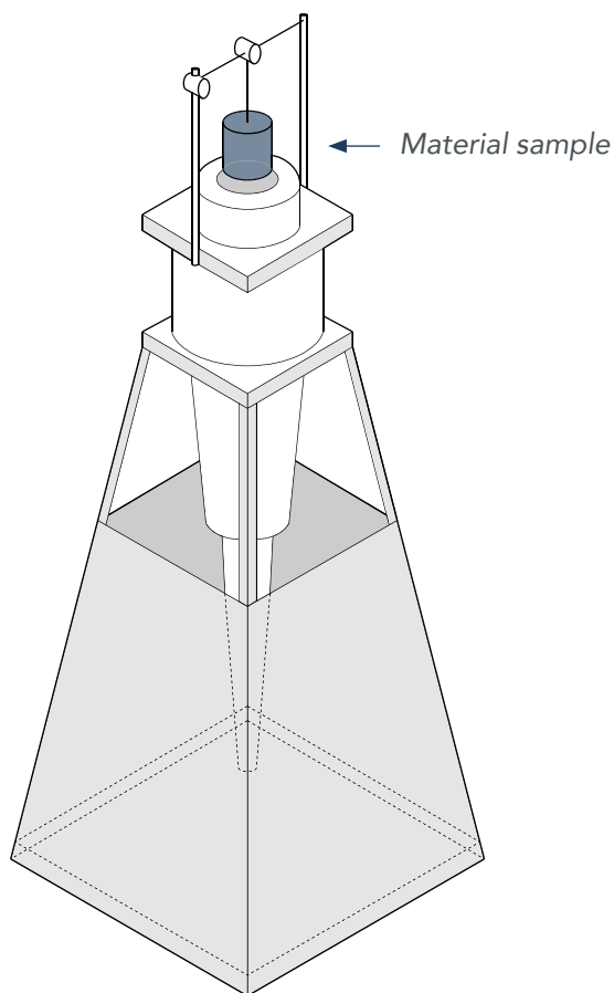
Non-combustibility tester
